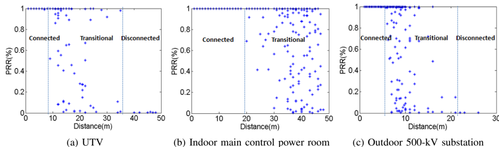
Fig. 1. Reception regions, in different smart grid environments (observed by TOSSIM simulation).
