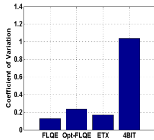
Fig. 7. Stability of Opt-FLQE, in the UTV environment.
